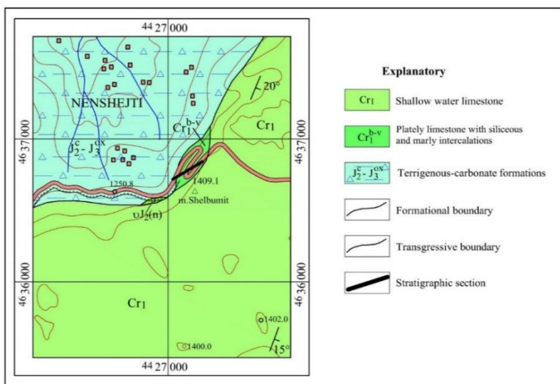
Fig. 3: Geological map of Mali i Shenjte (modified after Xhomo et al 2005).
