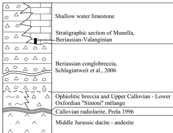
Fig. 5-1: Stratigraphic column of western Munella.
